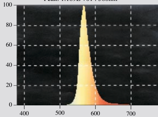
Fig. 3.2.3.5b - Spectral energy distribution of a narrow-band emitter
